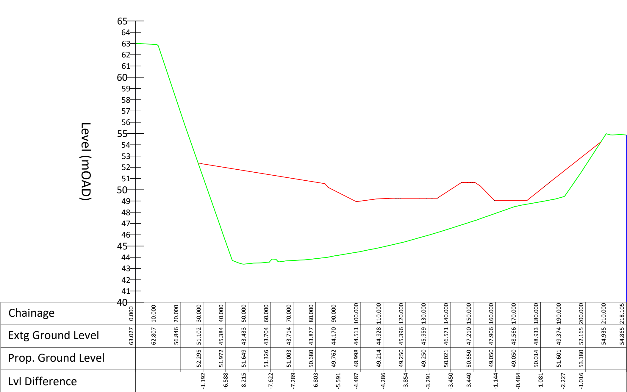
SECTION 5-5 Scale 1:1000H 1:200V
