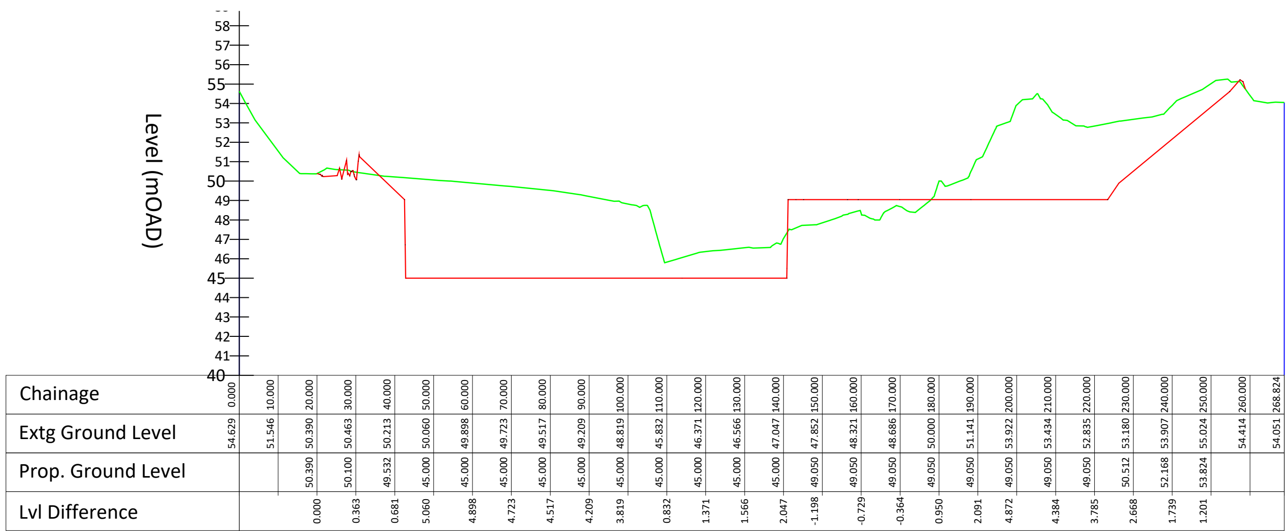
SECTION 6-6 Scale 1:1000H 1:200V
